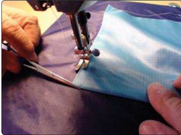
Figure 7-19. Corner fold.
