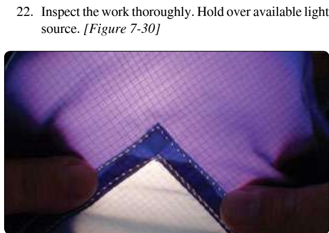
Figure 7-30. Patch inspection.
