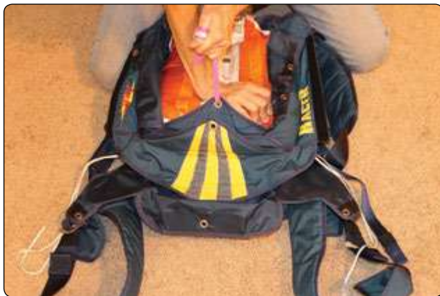
Figure 5-148. Close bottom sub flap.
