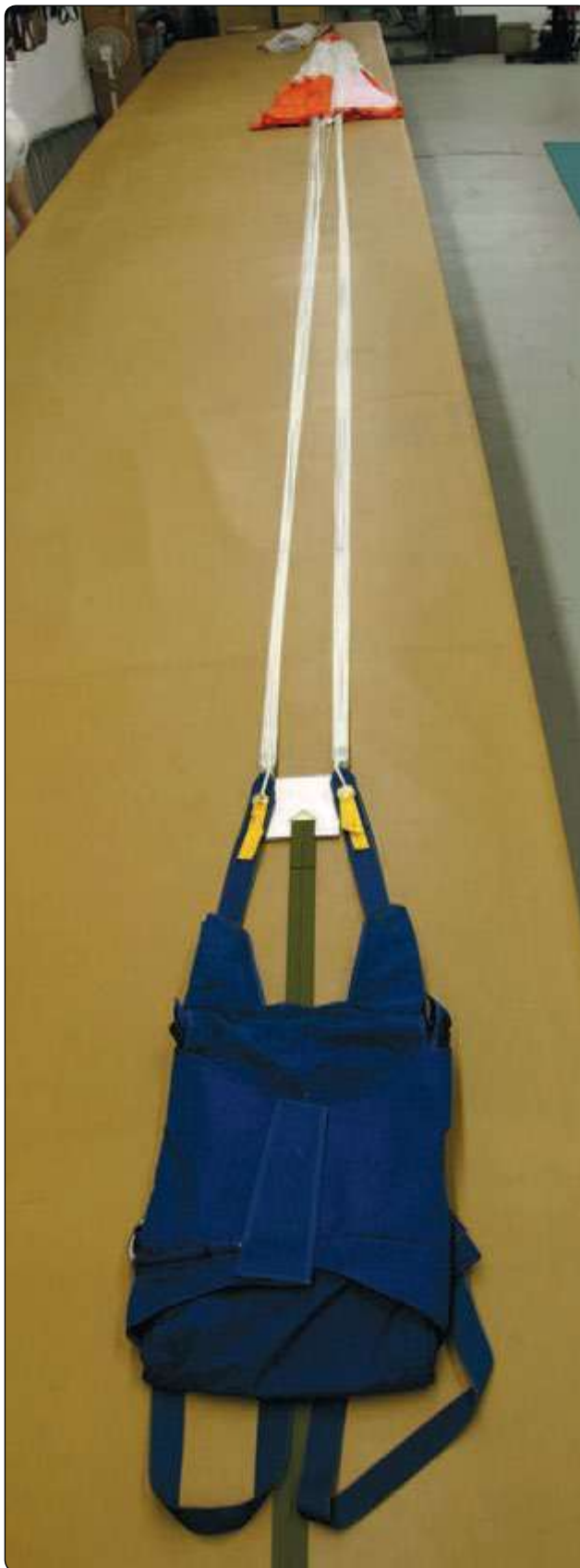
Figure 5-32. Round parachute assembly on packing table.
