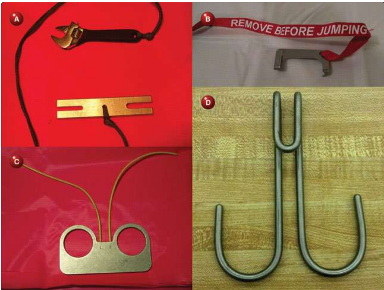
Figure 6-57. (A) link fork, (B) pull check tool, (C) tool used to maintain continuity of risers when removing main parachute from harness, and (D) Pro Pack hook.
